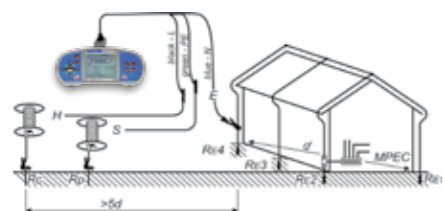
Circuits for three-wire measurement
